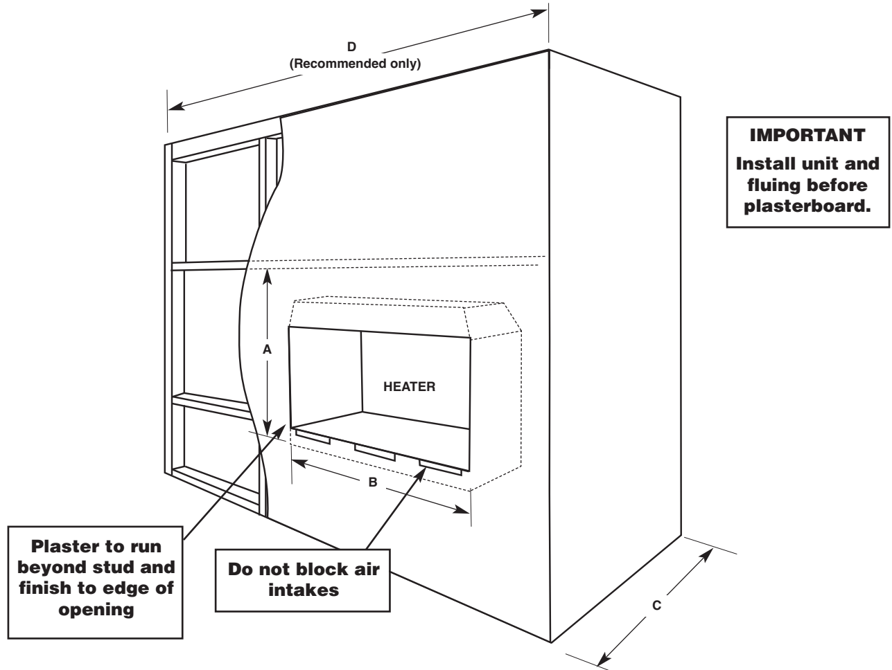
Frameout Dimensions (in mm)
